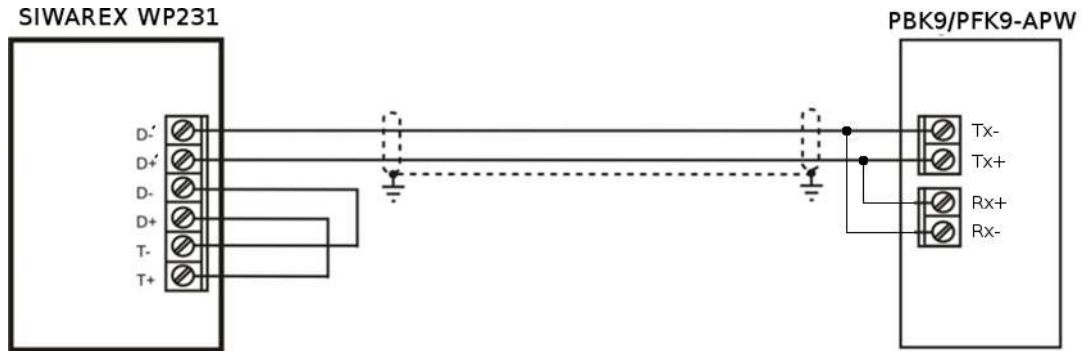
Figure 2: Connection diagramm
